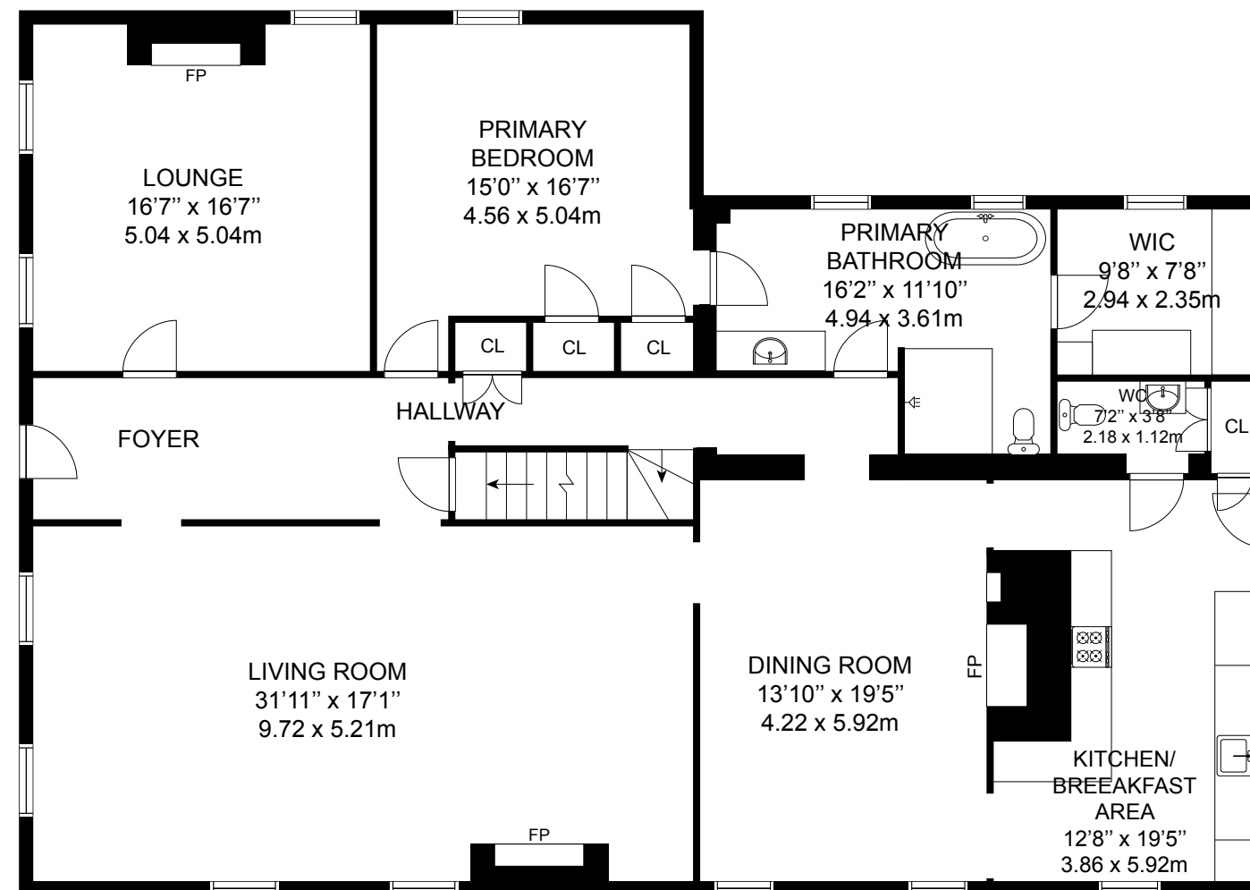
MAIN FLOOR
