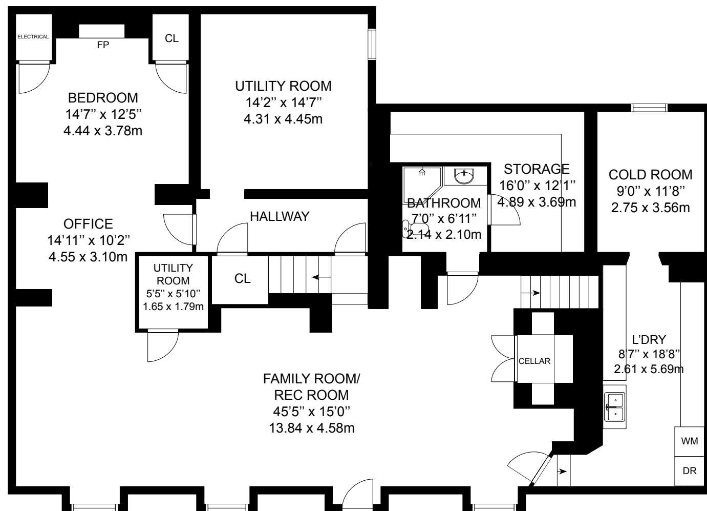
BASEMENT
