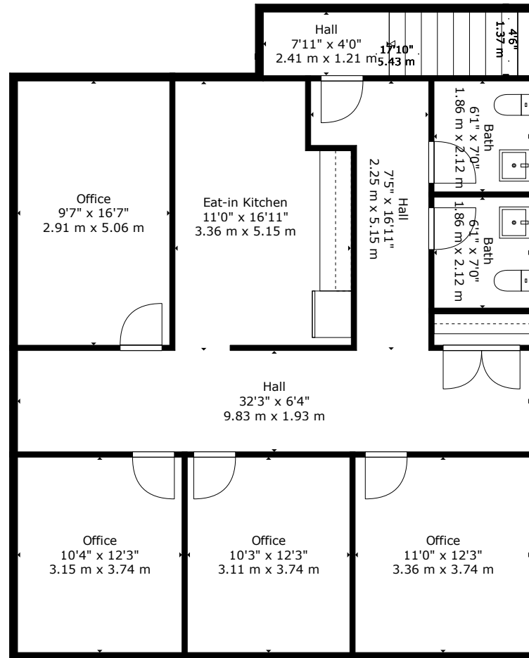
Floor 2
