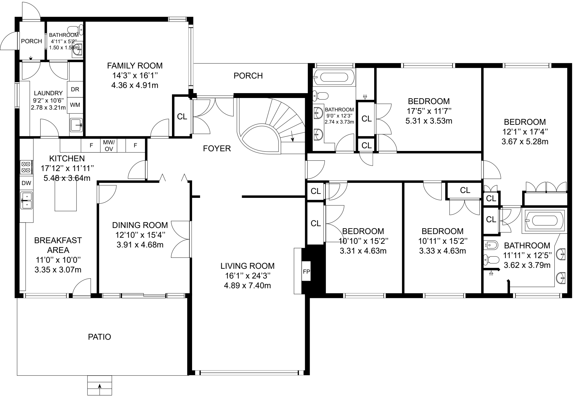
MAIN FLOOR
